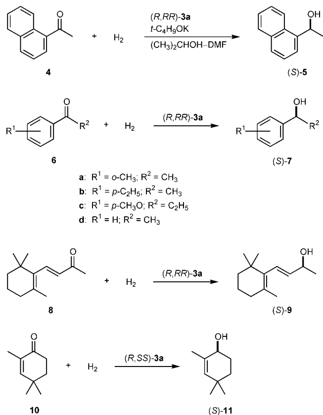
Scheme 2. Asymmetric hydrogenation of ketones.
