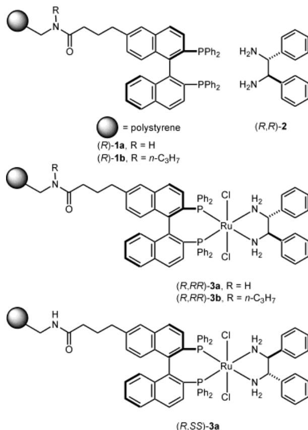
Scheme 1. Structures of compounds 1, 2, and 3.
